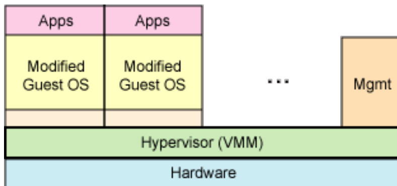
Para-virtualization
