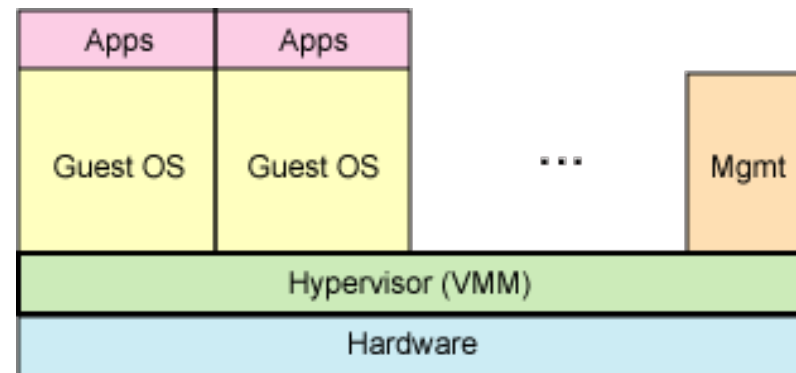
System-level virtualization
