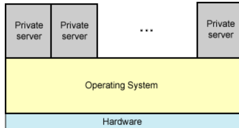
System-level virtualization
